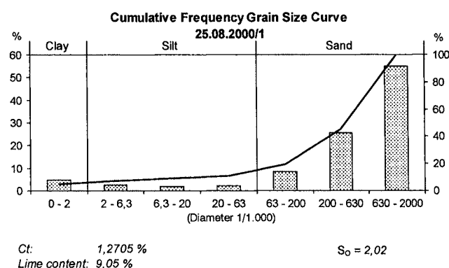
Figure 34. Ground- and lateral moraine matrix of the Late Glacial glacier filling of the Bar Nala (Stage I-III, cf. Tab. 1) in the area of the decimetres-, probably over 100 m-thick, inset of the medial moraine of Toltar, at the confluence of the then Baltar- and Kukuvar glacier components, 1200 m above the valley bottom of the Bar Nala (Kampire Dior group, S-side). Taken from an earth-pyramid wall, decimetres away from the bedrock. The portions of clay and silt amount to only c. 10%; a 90% portion is sandy. As it occurs in the lateral valleys of the glaciers, fluvial transport is probable. The arrangement of the columnar diagram is bimodal and thus typical of moraines: a primary maximum in the coarse sand (c.54%) and a secondary in the clay (c.5%). The sorting coefficient S_o = 2.02 , calculated after Engelhardt 1973: 133, evidences a glaciofluvial washing. There are also fluvially rounded SiO 2 -grains (2%); typical of moraine are the 98% sharply-edged crushed quartz-grains (cf. Fig. 6 No. 28). Cf. Fig. 35. Locality: Fig. 2 No. 95 (36°29' N/74°18'20" E, 3940 m asl). Sampling: M.Kuhle.
