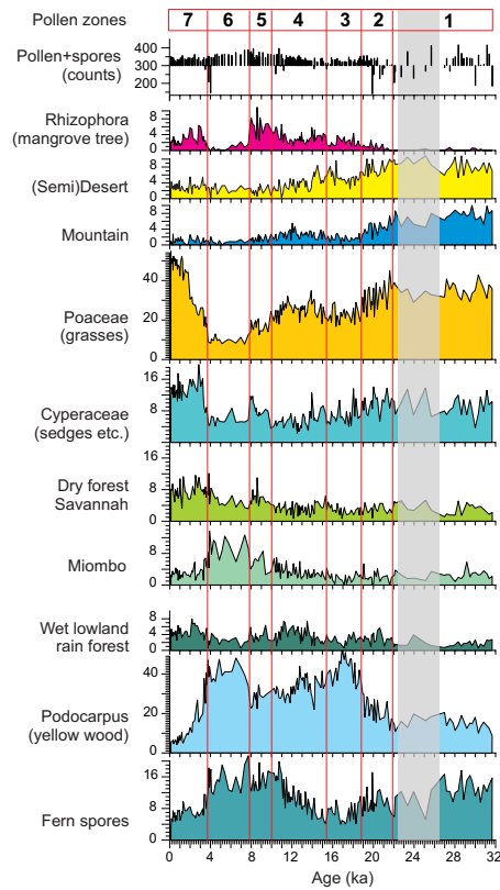
Fig. 4. Percentages of pollen taxa and groups (listed in Appendix A). Counts of total pollen and fern spores being the basis of the percent calculation are given on top.
