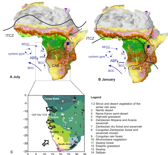
Fig. 1. Landcover of Africa (Bartholome et al., 2002), simplified phytogeography of southern Africa (White, 1983), ocean surface currents of the eastern South Atlantic (Shannon and Nelsson, 1996), and summer and winter position of important tropical frontal systems (Leroux, 1983). ITCZ, Intertropical Convergence Zone; CAB, Congo Air Boundary; ABF, Angola Benguela Front; SECC, South equatorial Counter Current; AC, Angola Current; BCC, Benguela Coastal Current; BOC, Benguela Ocean Current. (A): Austral winter (July) position of the ITCZ, CAB and ABF. (B): Austral summer (January) position of the ITCZ, CAB, and ABF. (C): Location of ODP Site 1078, general surface (air pressure level of 850 hPa) wind directions in austral winter (June, July, August), and biomes of southern Africa (see legend).
