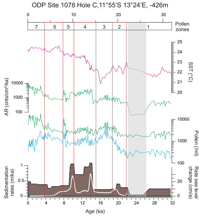
Fig. 3. From top to bottom. Pollen zones. Alkenone based sea surface temperatures (red line, upper right axis). Accumulation rates of total pollen per \text{cm}^2 and ka (green line, upper left axis). Total pollen concentration (green line) and Podocarpus pollen concentration (blue line) per ml sediment (middle right axis). Sedimentation rates in m per ka (shaded, lower left axis) and rates of sea-level change (line, lower right axis) after Fleming et al. (1998).
