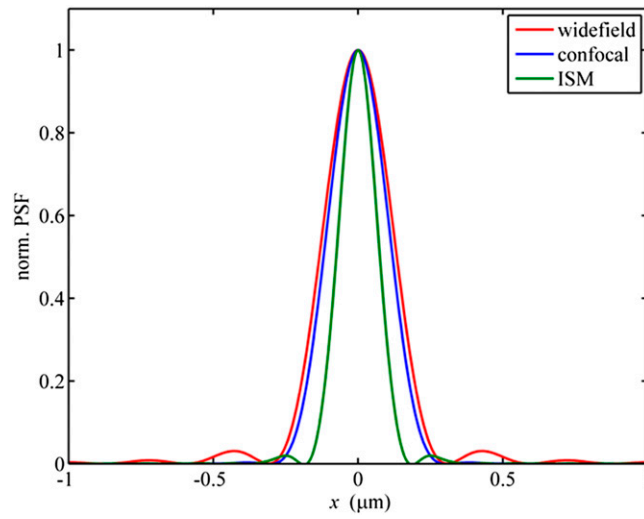
Fig. S2. Comparison of the lateral cross-sections of the PSF of a wide-field microscope, a confocal microscope, and an ISM microscope. The PSF of ISM is calculated after Fourier reweighting of its OTF, as described in the text.
