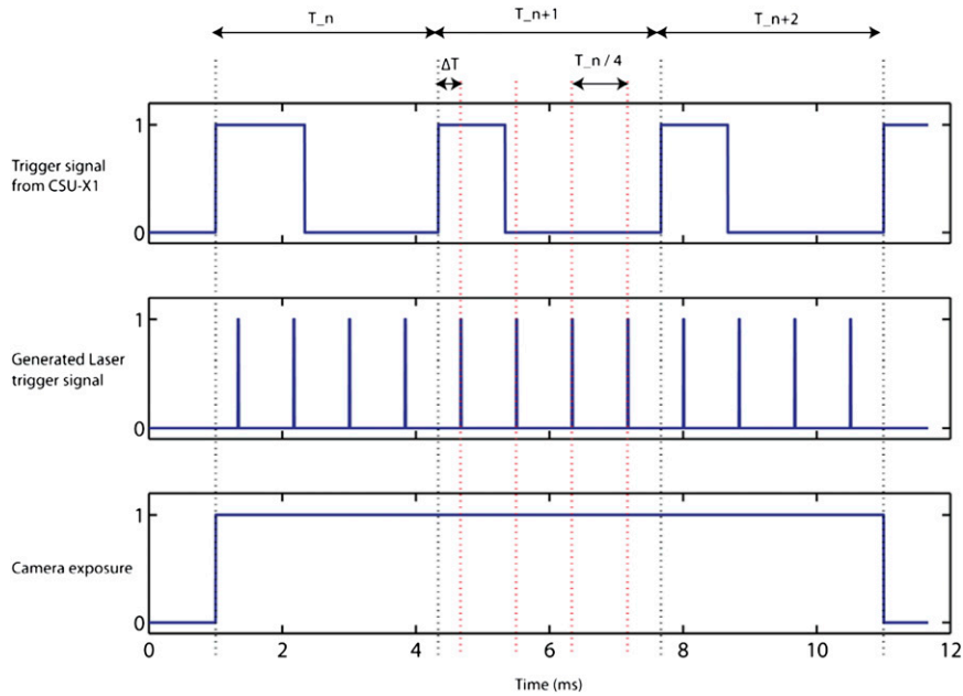
Fig. S3. Generation of trigger signals for CSD-ISM. See Synchronization and Data Acquisition for details.
