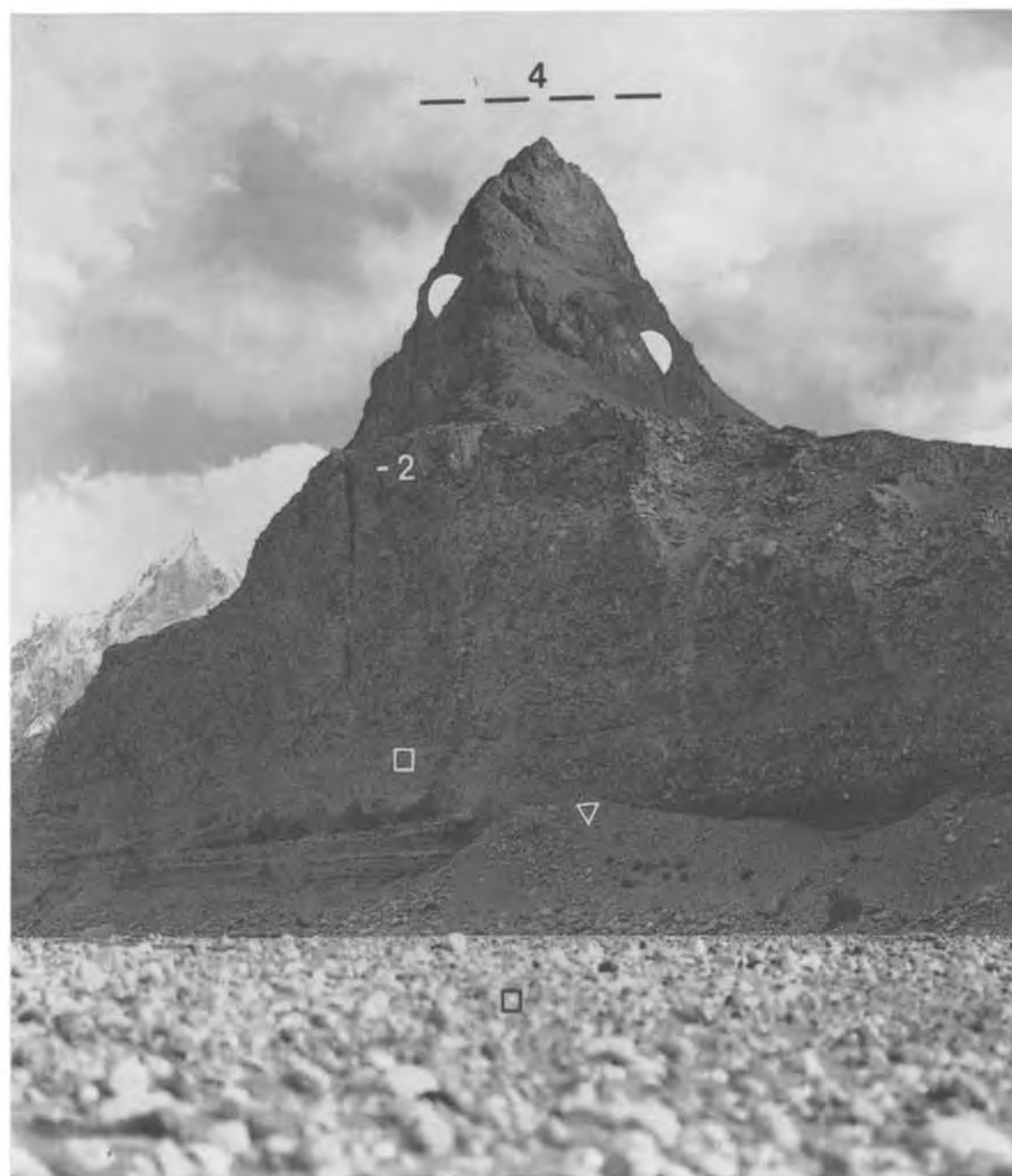
Fig 52 View of the 4730 m-high glacial horn (No. 4) made of limestone in the exit of the Muztagh valley from the drift floor of the Shaksgam valley (□ bottom) at 3900 m asl. In front the historic drift floor terrace No. -2 (Middle Dhaulagiri Stage 'VII). Viewpoint: 36°08'15"N/76°25'E (Fig 138 No. 13). Photo: M. Kuhle 31.8.86.
