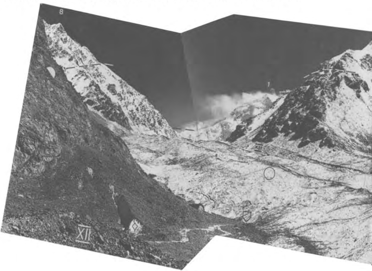
Fig 10 ▲ Panorama across the K2 glacier, taken from the orographic right-hand valley flank, at 5000 m asl, at the half-way point of the ice stream's length; from SSE (No. 1 = K2, 8617 m) via No. 2 (6800 m peak), No. 3 (c. 7000 m-high N-satellite of the Chongtar Peak), No. 4 (more than 7000 m-high N-satellite in Chongtar Group); No. 5 (c. 6000 m-high sub-summit in the northern Chongtar Group) via W with No. 6 (an ESE spur peak of the 6540 m summit), via No. 7 (c. 6000 m-high peak between 6540 m and 6040 m peak) towards NNW to the (No. 8) Aghil Mountains main ridge beyond the Shaksam valley, which rises up to 6750 m there. On the mountain flanks above the still dendritic valley glacier system of the K2 glacier with its side glaciers (below No. 4) the highest established prehistoric glacier levels are marked (---). Due to steepness, frost weathering and local denudational and erosive processes on the valley flanks the roughening of the walls down to the present glacier level is extremely severe, so that next to no rock abrasions and polishings are preserved (●). The increasingly heavy cover of surface moraine is due to the horizontal and vertical distance of the ELA, which is now running at the foot of the wall of K2 at about 5200 m asl. Viewpoint: 35°58'N/76°29'E. Photo: M. Kuhle 3.10.86.
