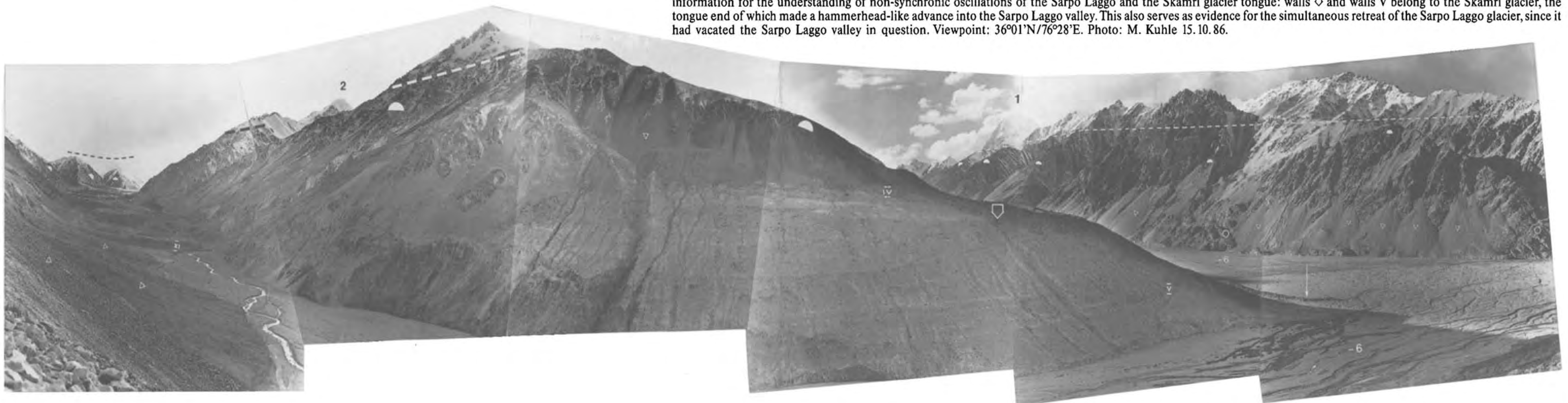
Fig 44 ▲ View of the Sarpo-Laggo glacier from an altitude of 4380 m asl, facing SSW up to the 6544 m peak (No. 1) and on to facette-like, down-worn glacigenic truncated spurs and cusate areas (●●) (Fig 138, No. 7). The Ice Age filling of the transgression glacier covered the relief up to and beyond such ridge peaks (---). The Sarpo-Laggo glacier is in the process of retreating. Its dendritically-branching tributaries (→), each with two side moraines coalescing with others to form numerous median moraines in the glacier tongue, have brought down so much scree that end moraines (■) have been deposited. The form of their embayment, however, is largely due to their core of dead ice. They were formed when the ice retreated - ie not accumulated, but classic dumped end moraines. Viewpoint: 36°00'N/76°22'E (Fig 138, No. 4). Photo: M. Kuhle 17.10.86.
