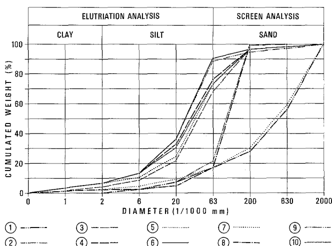
Fig 55 Cumulative Frequency Grain-Size curves from different clastic materials from the Karakoram region. Quaternary sediments in the arid high-mountain environment between the Aghil main chain, over the western Kuenlun to the northern piedmont areas leading down into the Tarim Basin (37°46'N/36°24'N; altitud between 1480 and 3900 m asl), sub-2 mm fractions. Curves 2 and 8 show grain-size distribution from widespread, 1 to 2° inclined glaciofluvial fans on the piedmonts at 1480 m, more than 60 km away from the solid rock of the mountains. Curve 6 (till; 3740 m) shows the same characteristics as curve 9 (mudflow). In both cases the source rock is the Kuenlun granite, and the distance of transport amounts 15 km. Curves 1 and 5 are characteristic for alluvial terraces at the bottom of the Yarkand Valley (3800 m asl); the material contains granites from the Kuenlun slope and metamorphic rock (clay, silt and sandstones) from the Aghil slope.
