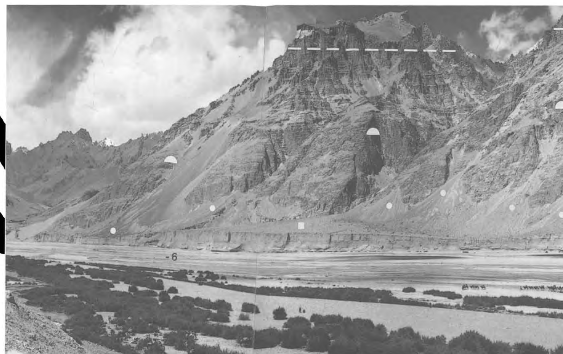
Fig 39 ▲ Taken at 4120 m asl; view from the orographic left-hand flank of the Shaksgam valley towards the NW to the opposite valley flank; being part of the Aghil mountains it is constructed from horizontal dolomite strata (Fig 138, No. 23). It is a trough flank which is characterized by glacial band abrasion and polishing (●); the ice scour limits (----) extend to c. 1200 m beyond the edge of the trough. Talus cones and fans (●) were built up within a few thousand years after glaciation, and simultaneously undercut by the bed of washed drift (-6). Viewpoint: 36°08'50"N/76°36'E. Photo: M. Kuhle 30.8.86.
