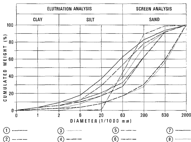
Fig 66 Cumulative frequency grain-size curves from different clastic materials from the Karakorum region. Grain-size curves of alluvial and glaciofluvial sediments. Samples 5 and 8 are from very large gently sloping ( 1^\circ ) glaciofluvial fans on the piedmont. The material is polymictic. The distance transported amounts to more than 100 km (3850 m asl). Curves 1, 2, 4 and 7 show gravel deposits with differing admixtures of talus cone material on the bottom of a narrow Kuenlun valley. The granite and metamorphic detritus has been transported 10 km at the most. Curves 3 and 6 show also well-graded gravel deposits consisting of granitic and metamorphic detritus after transport of up to 100 km (middle Yarkand valley; 3800 m asl).
