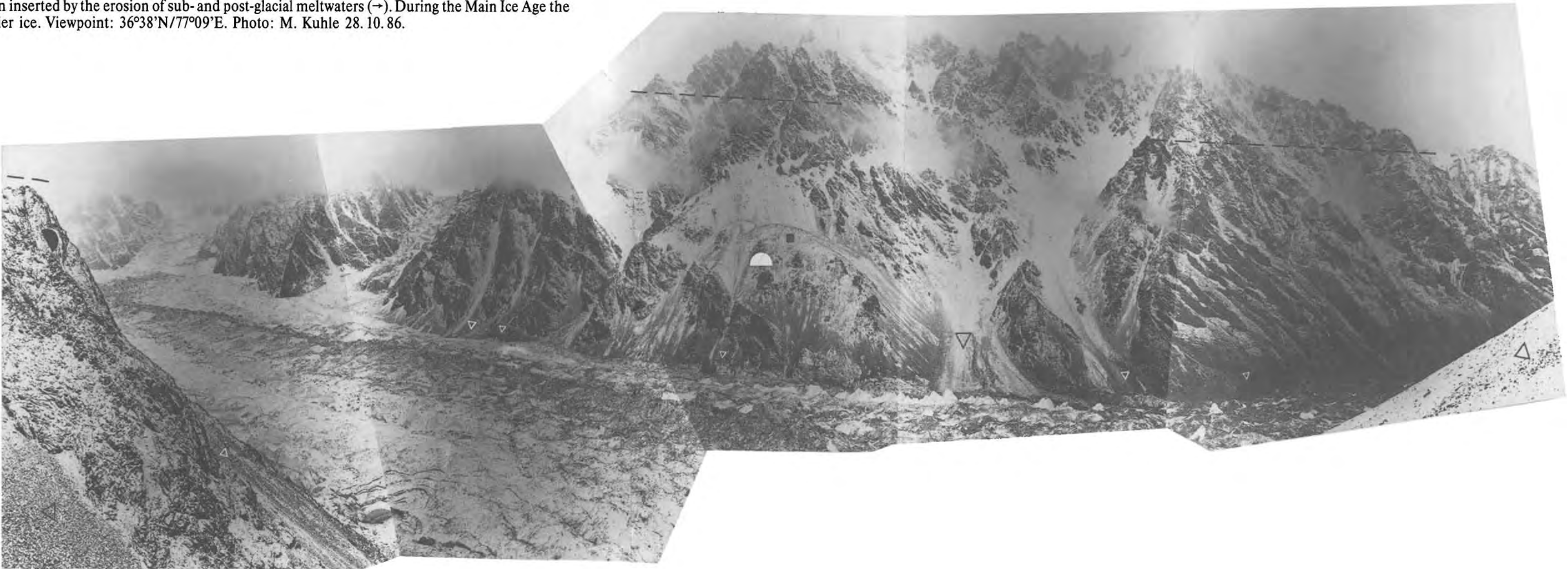
Fig 27 ▲ View from the drift floor of the Shaksgam valley (□ below) which continues to undergo annual working-through, facing SSE towards some satellites of the 6210 m-high peak (No. 1), a spur peak of the Karakorum system, and into an orographic left-hand side valley (Fig 138, beneath No. 21). At the valley head a glacier hangs down (○). Thanks to its extreme steepness as a glacial cut, or gorge-like trough, the side valley was partially buried by post-Late Glacial talus cones. In the area of the confluence with the main valley, perfectly preserved flank abrasions and polishings (●) suddenly set in. They are evidence of an extremely thick prehistoric infilling of ice. The former glacier level (----) can be established with the aid of an ice scour limit. Viewpoint: 4020 m asl, 36°08'N/76°35'E. Photo: M. Kuhle 1. 9. 86.
