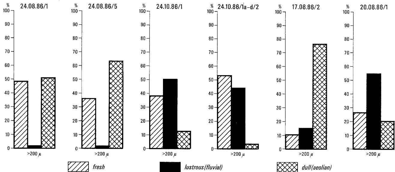
Fig 56 Surface texture of sediment grains greater than 200 \mu m. Samples 24. 8. 86/1 and /5 (cf. Fig 66, Nos. 1, 7) show the characteristics of very briefly transported (less than 10 km) gravel and talus material from a canyon in the Kuenlun: fresh, angular grains (I) have the same portion as the aeolian grains (III), while the fluvatile-polished material (II) is almost completely lacking. Samples 24. 10. 86/1 and 24. 10. 86/1a-d/2 were all taken from outwash terraces in the semi-arid Yarkand valley; however, the distance to the source areas varies. With a greater transport distance, sample 24. 10. 86/1 shows a predominance of group II (fluvial grains), followed by the aeolian material (III) and has only a very small portion of group I. Due to the comparably long fluvatile transport of sediment 17.08.86/2 (cf. Fig 55, No. 8) group I (angular, fresh) takes almost no part in it. In group III aeolian transport predominates which is typical for sediments of 200 \mu m in full-arid environments. Sample 20. 8. 86/1 (cf. Fig 55, No. 6) shows the characteristics of a till at a distance of up to 15 km from the source area. The fluvatile-polished grains (II) are predominant; it cannot be determined on each grain whether the group I grains must attributed to normal weathering or to glacial erosion and transport, but most of this substratum has been pounded and fractured by the glacier and shows crescent-shaped chattermarks on the grain surfaces. The aeolian material (III) still has a portion of 20% and seems to have been blown from a distance.
