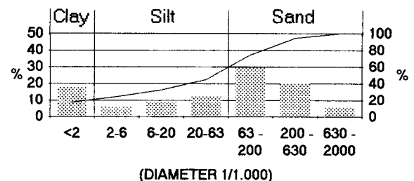
Figure 14. Ground moraine matrix from the area of the Last Glacial (LGM) Laurentide Ice Sheet in the Canadian North America, taken for comparison with prehistoric Tibetan ground moraines. Locality: Canadian prairie at Moose Jaw, 40 km N of Old Wives Lake and 85 km ESE of Lake Diefenbaker. Cf. Figures 6, 8 and above all 13. (Sampling: M. Kuhle.)
