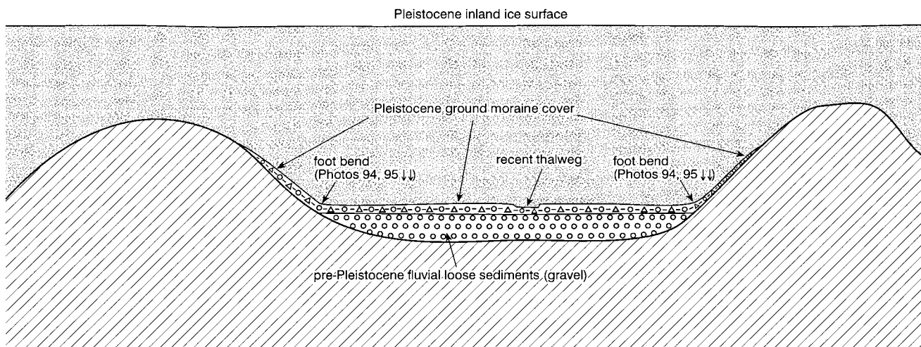
Figure 23. (cf. Photos 94 and 95). Ground moraine cover over pre-glacial (pre-Pleistocene) purely fluvial gravel bodies.
