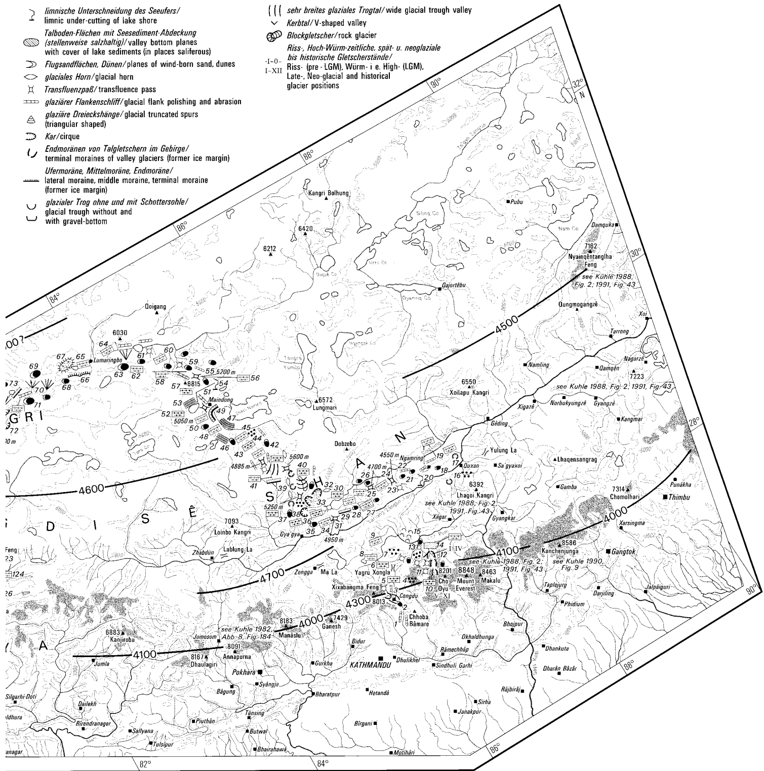
Figure 2. Quaternary-geological and glaciogeomorphological map of South-, Central- and West Tibet.
