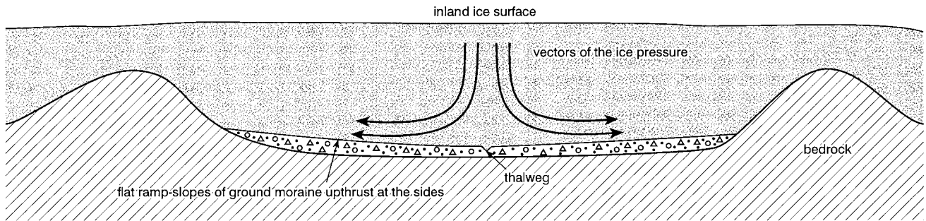
Figure 20. On the genesis of flat glacial ramp-slopes in High Glacial ground moraine.
