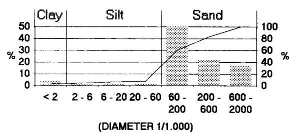
Figure 21. Ground moraine matrix from Central Tibet (see Photo 85 near the right margin, background); sampling at 4280 m (aneroid measurement at high pressure; actual height about 4500 m asl); Figure 2, No. 59; 31°56' N/85°04' E; taken from a depth of 0.2 m. Despite the rather insignificant peak in the clay of ca. 4%, the typical bimodal course of the curve is evident. The coarser fine grain peak of 50% in the fine sand is very pronounced. It points to a relative coarse crystal structure of the bedrock from which this material has been abraded. For the morphometry of the quartz grains, cf. Figure 5 diagram 30.08./1. (Sampling: M. Kuhle.)
