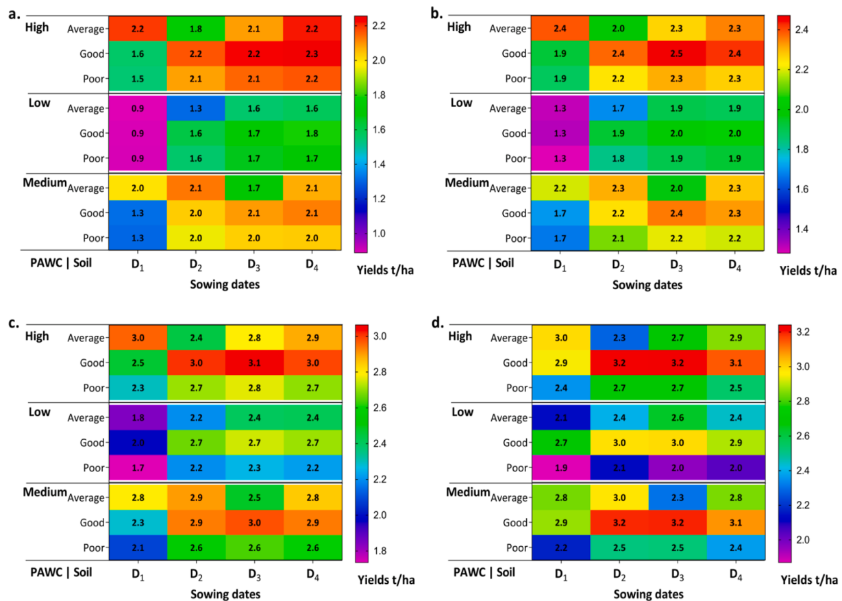
Fig. 5. Average simulated maize yields ( \text{t ha}^{-1} ) for different soil organic carbon levels (average, good, and poor), different levels of PAWC (high, low, and medium), and different sowing dates (i.e. according to onset definitions of Raman's ( D_1 ), Modified Sivakumar's ( D_2 ), Yamada's ( D_3 ), and Liebmann's ( D_4 )) in main the four different climatic zones i.e. (a) Sahelian, (b) Sahelian-Soudanian, (c) Soudanian-Sahelian, and (d) Soudanian-Guinean.
