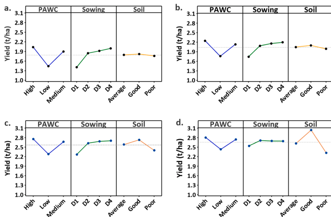
Fig. 4. Main effects plots of the maize yield determinant factors i.e., PAWC, sowing dates, and soil organic carbon in different climatic zones i.e. (a) Sahelian, (b) Sahelian-Soudanian, (c) Soudanian-Sahelian, and (d) Soudanian-Guinean.
