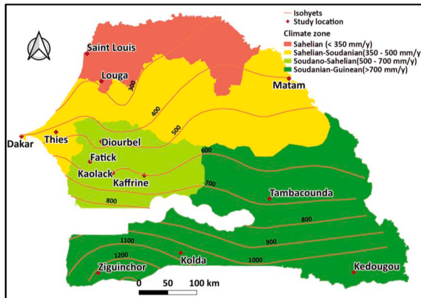
Fig. 1. The map of Senegal showing locations in different rainfall zones in the study area. The average annual rainfall on which the “climate zonation” was based was computed for the period 1981 – 2020.
