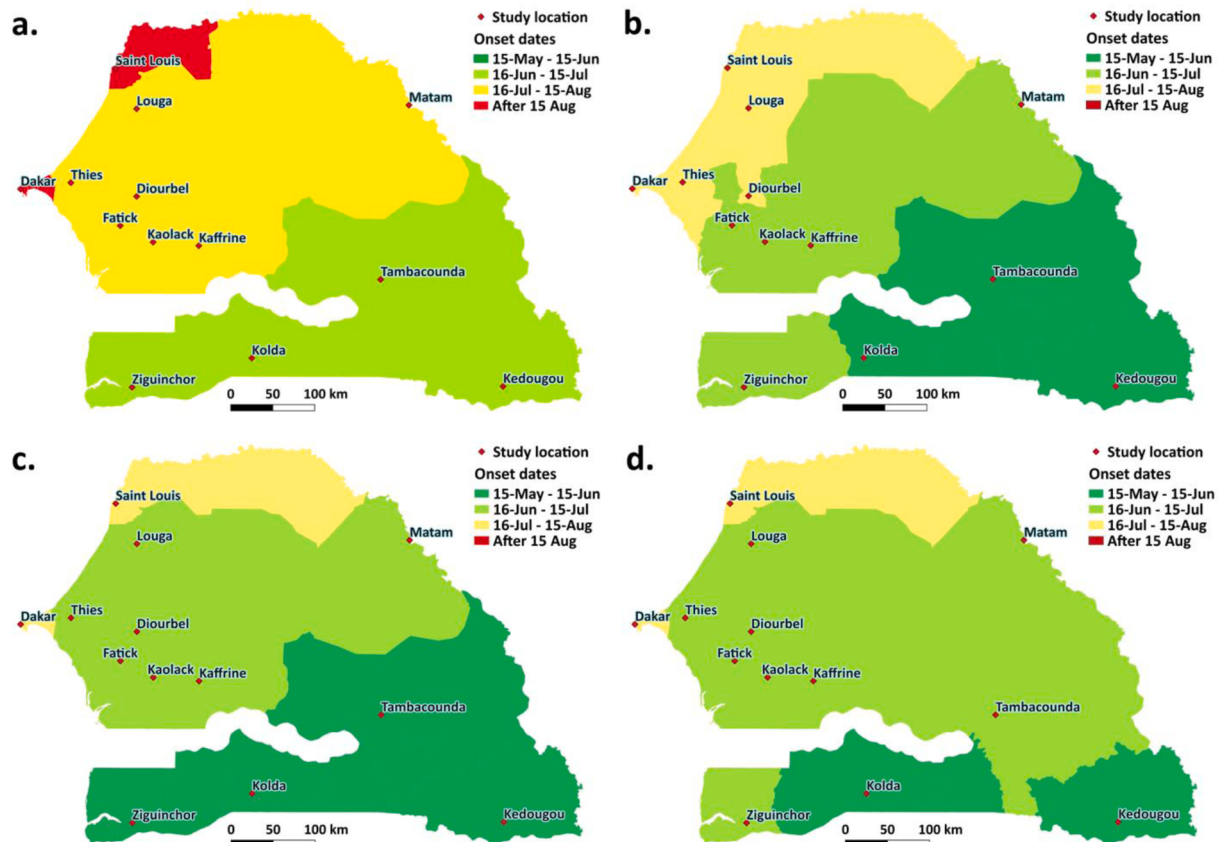
Fig. 3. Onset dates as defined by the four definitions i.e. (a) Raman's ( D_1 ), (b) modified Sivakumar's ( D_2 ), (c) Yamada's ( D_3 ), and (d) Liebmann's ( D_4 ) per definition in the study locations from 1981 to 2020.
