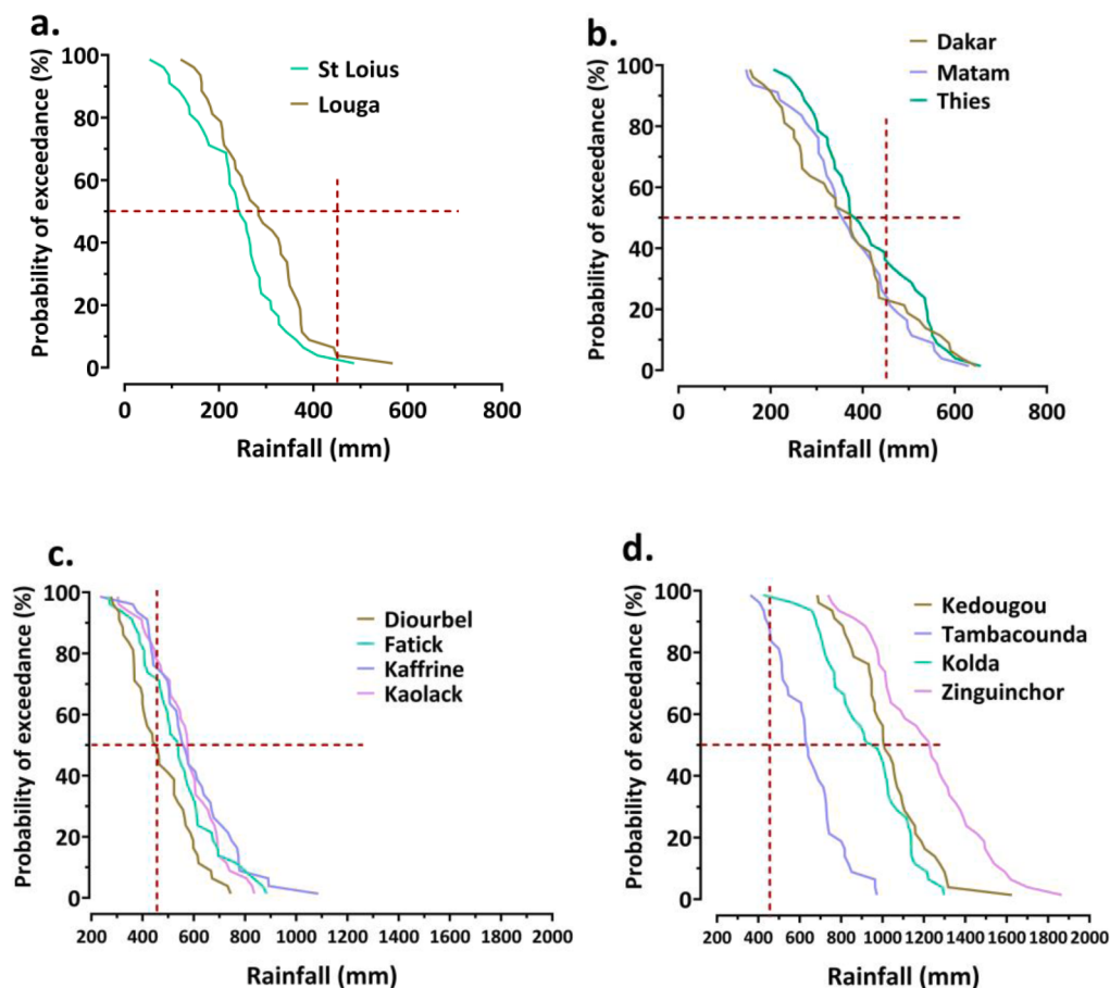
Fig. 2. The seasonal rainfall probability of exceedance charts for the locations in the (a) Sahelian, (b) Sahelian-Soudanian, (c) Soudanian-Sahelian, and (d) Soudanian-Guinean climatic zones from 1981 to 2020.
