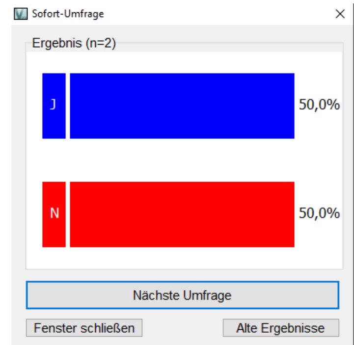
Windows-Desktop-Client
